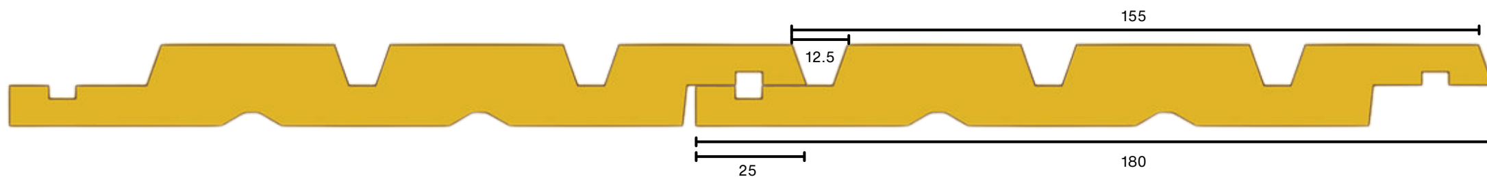
MD57 Vertical Shiplap 180/18.5mm 155mm Cover
