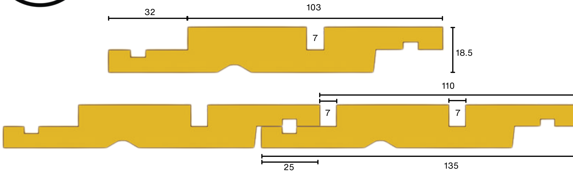
MD58 Vertical Shiplap 135/18.5mm 110mm Cover
