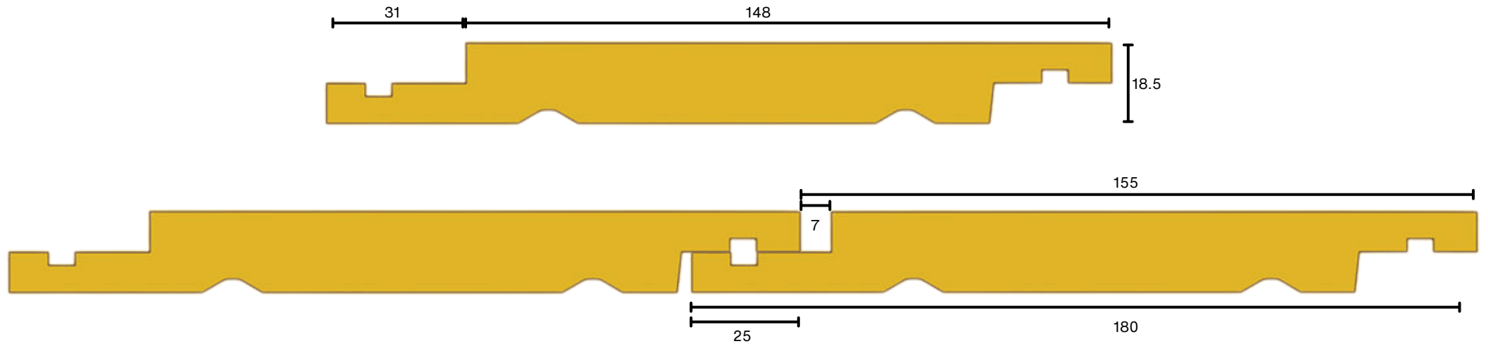
MD56 Vertical Shiplap 180/18.5mm 155mm Cover
